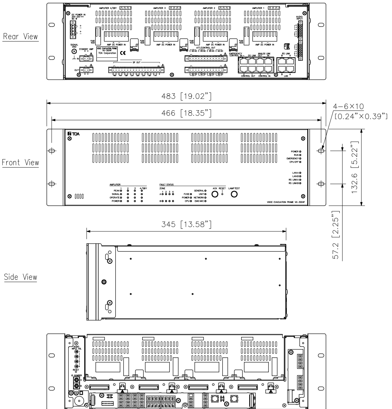
Front view without front panel
