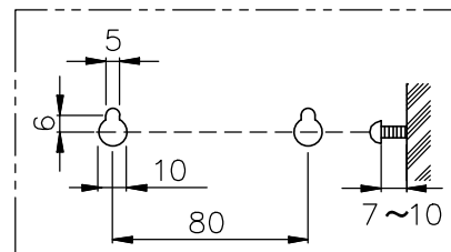
Hanging holes dimension diagram
