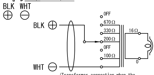
Wiring diagram
