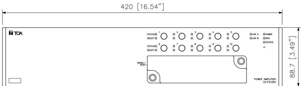
Front View
