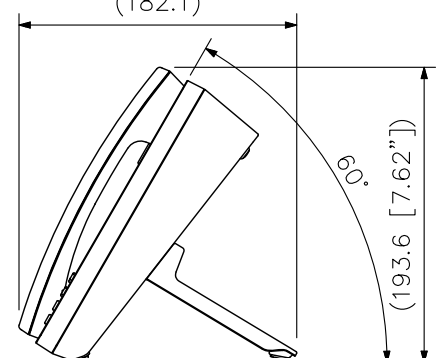
Stand Installation View (60° upward)
