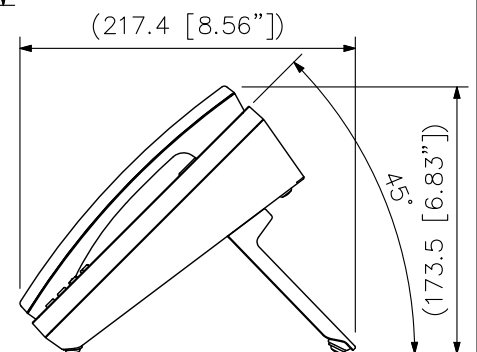
Stand Installation View (45° upward)
