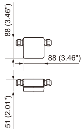
[Terminal box (Accessory)]
